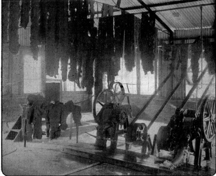
PLATE I (a).—TREATMENT OF THE FIRST COAGULUM OF LATEX; MACHINE FOR WASHING IT.
